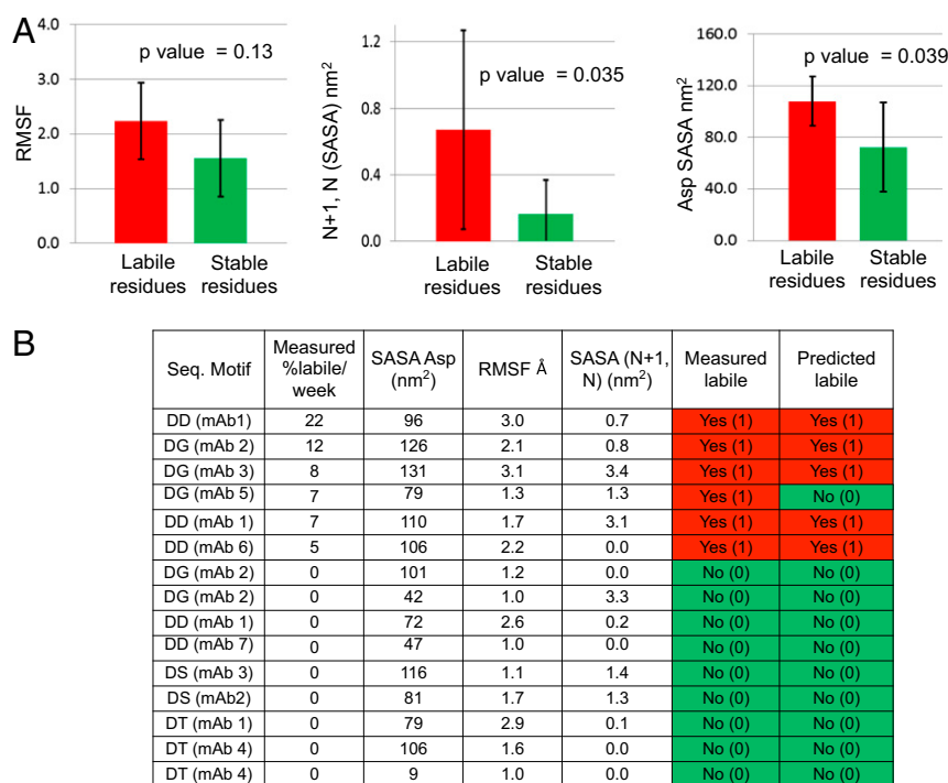
Fig. 4. (A) Comparison of the average and SD of various properties, i.e., SASA, RMSF, and SASA ( n + 1 , N ), extracted from MD simulations for labile group (red) vs. stable group of Asp residues (green). Calculated P values are shown on each plot. (B) Outcome of the logistical regression to enable prediction of labile vs. stable Asp sites. Logistic regression was performed using SASA, RMSF, and SASA ( n + 1 , N ) as independent variables and the binary rate output as the dependent variable. All sites were assigned a value of 1 or 0 for labile and stable sites, respectively, based on a cutoff value of Asp degradation rate of 2.5%/wk at pH 5.5. Labile residues are shown in red and stable residues are shown in green. The predicted outcome was generated using the binary logistic model as described in the text. The model was validated using the LOOCV approach.
